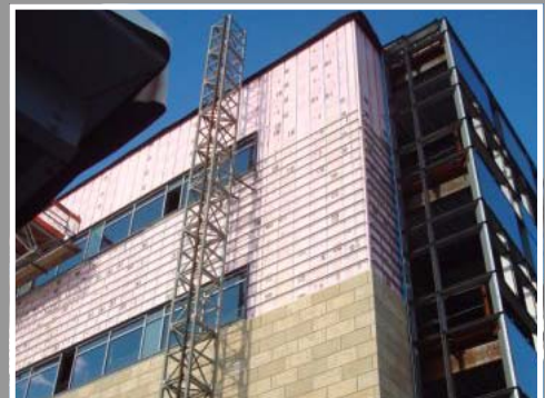
Step 6: Clip Stone on to the Gridworx Channels
